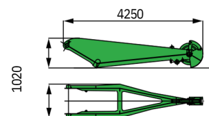
Auxiliary jib S24.1 (510 kg) Load rating 24.0 t
